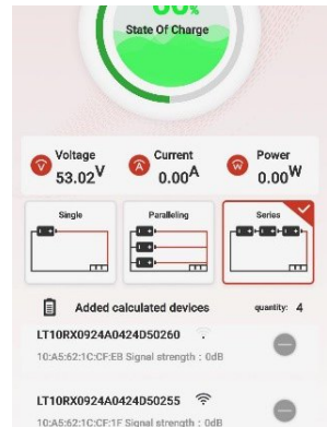
Series Configuration
