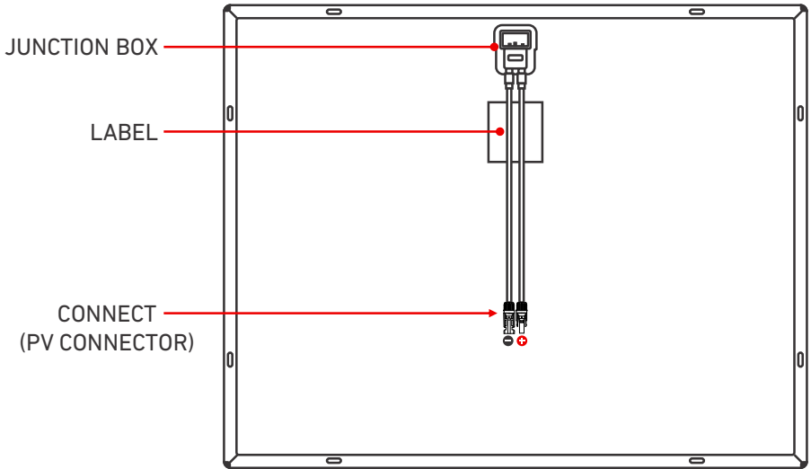
BACK VIEW
